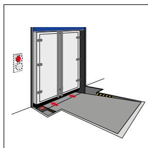
6. Extend lip to cover gap
