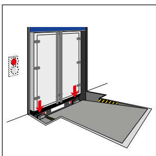
5. Bumpers go down
